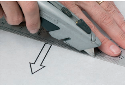
To cut tiles, score on reverse
